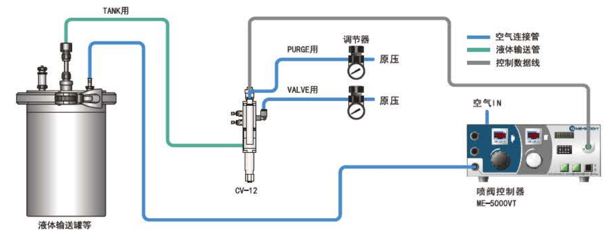
■涂层喷阀 CV-12
